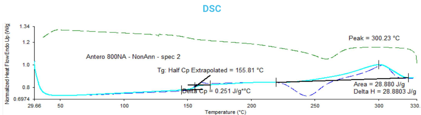
Figure 1: 2nd Heating Scan, DSC, for Antero 800NA
